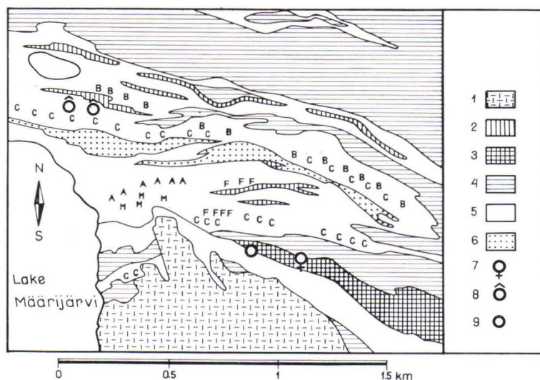
FIG. 2. Geology and ore deposits of the Ilinjärvi field. 1. Orijärvi granodiorite, 2. skarn, 3. cordierite-anthophyllite rock, 4. amphibolite, 5. leptyte, 6. porphyritic leptyte (A = andalusite, B = biotite, C = cordierite, F = anthophyllite and M = muscovite as porphyroblasts and as the characteristic mineral of leptyte), 7. Orijärvi copper-zinc deposit, 8. Ilinjärvi zinc-lead deposit, 9. Nygruva pyritic ore.
